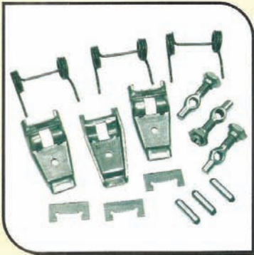
JEEP CLUTCH LEVER KIT
